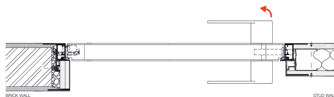
INSTALLATION PULL EU RIGHT
