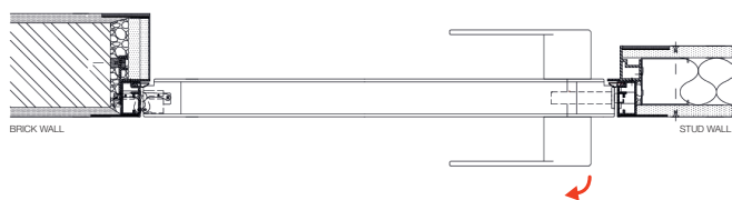
INSTALLATION PUSH EU LEFT
