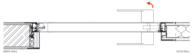
INSTALLATION PULL EU RIGHT
