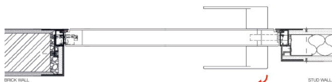
INSTALLATION PUSH EU LEFT
