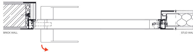
INSTALLATION PUSH EU RIGHT
