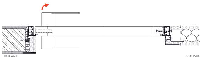
INSTALLATION PULL EU LEFT
